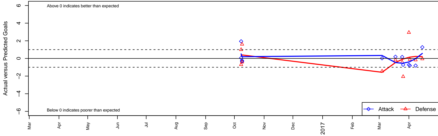
Valley Thunder SC G03 Dots are actual minus expected GF (blue circles) and GA (red triangles). Blue line is smoothed change in attack strength. Red is smoothed change in defense strength.
